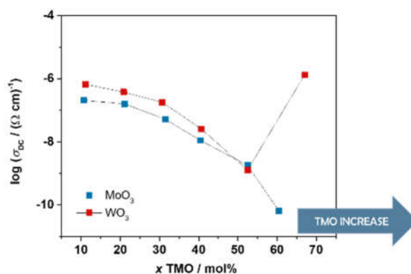
Figure 1. DC conductivity at 30°C as a function of TMO content for glasses from (60-x)\text{V}_2\text{O}_5-x\text{TMO}-40\text{P}_2\text{O}_5 series.
