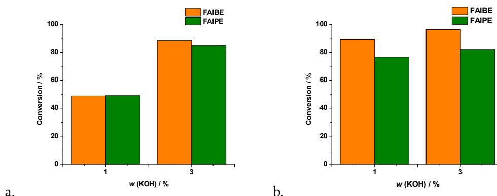
Figure 1. The influence of the mass fraction of KOH on reaction conversion of FAIBE and FAIPE, when the molar ratio of the reactants is 6:1 (a) and 12:1 (b).
