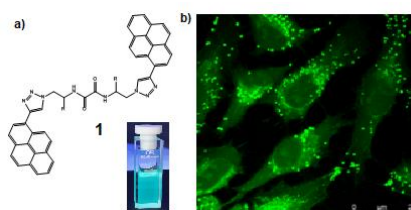
Figure 1. (a) Structure of 1 (R = iso-butyl) and (b) confocal image of MDA-MB-435S cells incubated with 1 .
