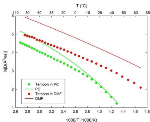
Figure 1. Curves of Tempone diffusivity and self-diffusion coefficients for PC and DMF
