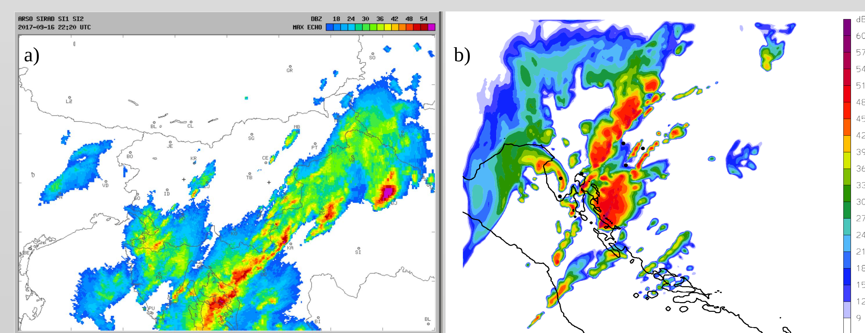
Figure 8: (a) Measured (22:20 UTC) and (b) modelled (23:00 UTC) maximum radar reflectivity (dBZ) . Spots with maximum radar reflectivity above 40 dBZ occur; some of these areas can be linked with observed hail (fig 6). The modelled maximum radar reflectivity has slightly higher values and affects an area that is larger and NW from the observed area. It consequently predicts widespread hail.
