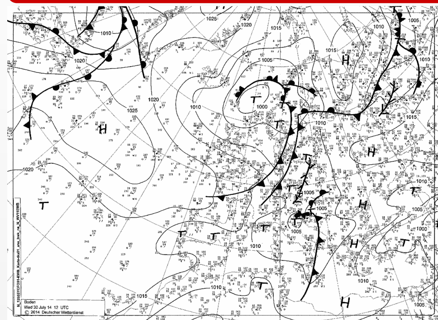
Figure 1: Surface diagnostic chart at 12 UTC on 30.7.2014 for Europe (Source: wetter3.de). Croatia is under influence of low pressure system. Winds are moderate and from E to SE directions.
