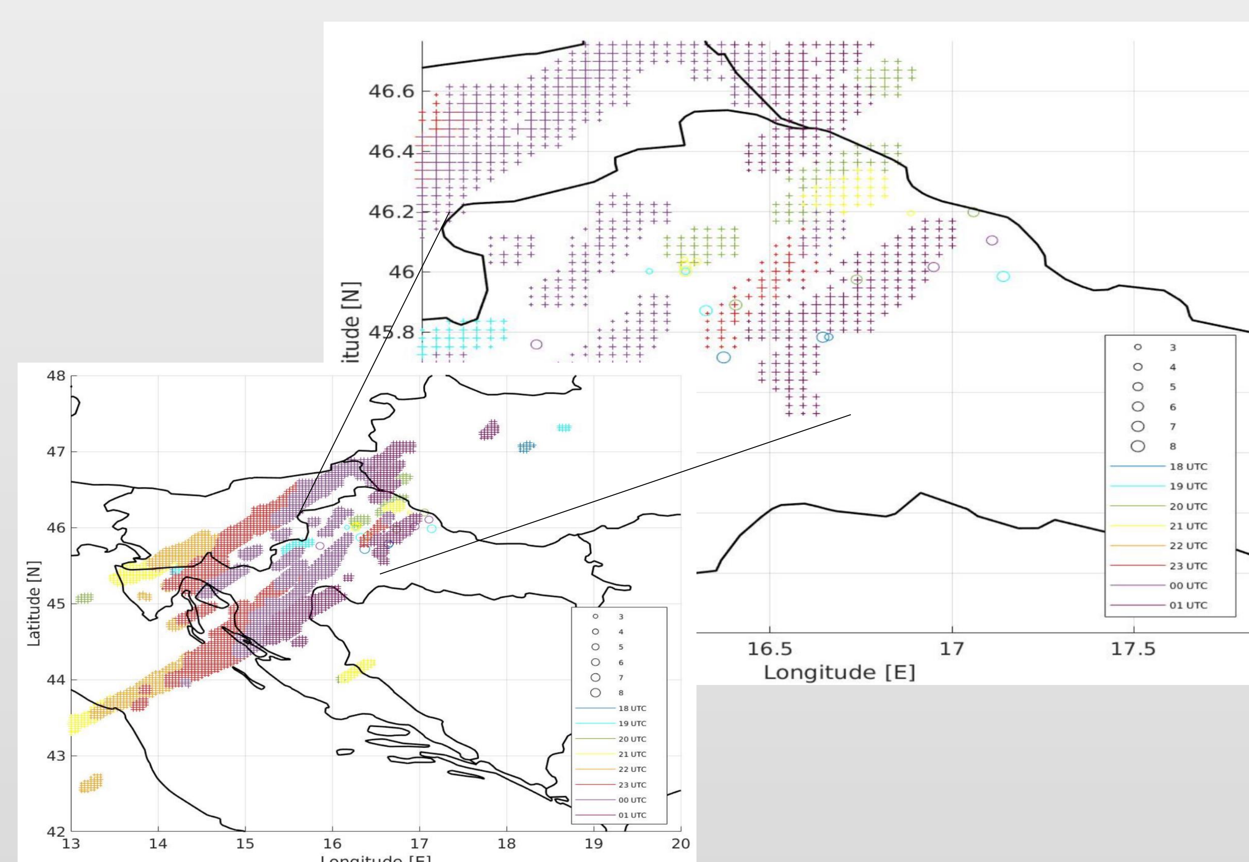
Figure 6: Modelled and measured maximum hail diameter . Colours represent UTC time, size of the crosses and circles modelled, i.e. measured max hail diameter classified into hail categories. Model didn't capture temporal characteristics of the observed hail and took into account too large an area.
