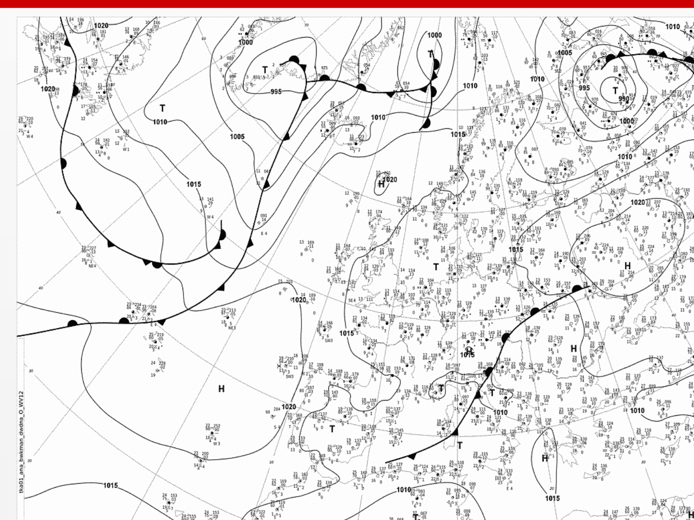
Figure 3: Surface diagnostic chart at 18 UTC on 16.9.2017 for Europe (Source: wetter3.de). Target area is under influence of low pressure system. Winds are weak from S to SW directions.
