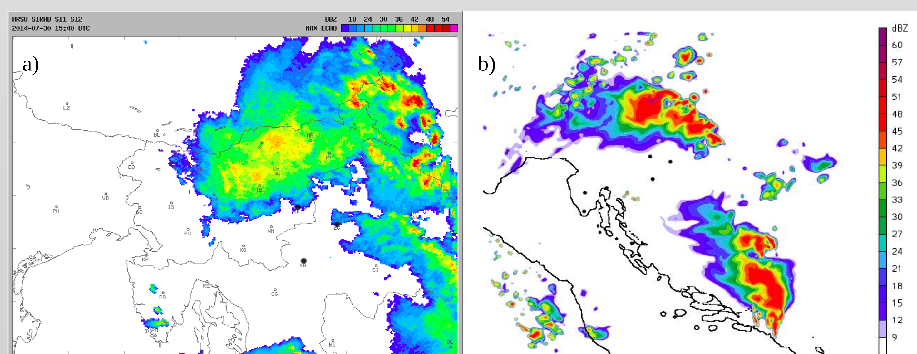
Figure 7: (a) Measured (15:40 UTC) and (b) modelled (16:00 UTC) maximum radar reflectivity (dBZ) . In northern Croatia, spots with maximum radar reflectivity above 40 dBZ occur. We can link some of these areas with observed hail (fig 5). The modelled maximum radar reflectivity affects much larger area and has slightly higher values. It consequently predicts widespread hail.
