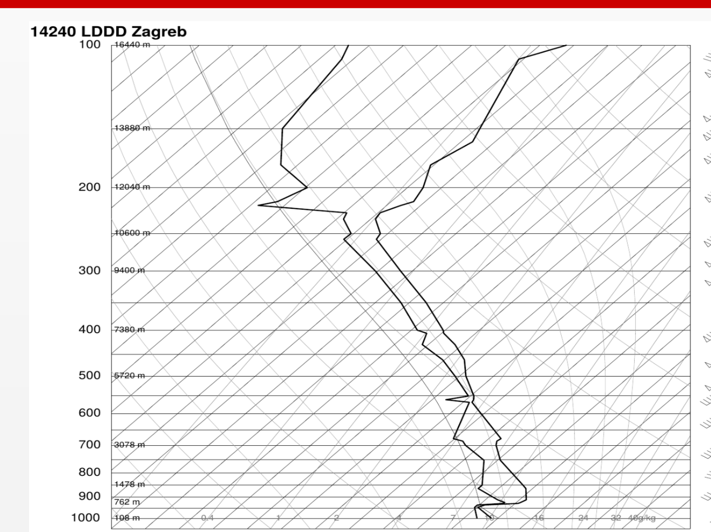
Figure 4: Sounding from Zagreb, Croatia (30.7.2014, 12 UTC) . CAPE = 0.0 J kg-1, LI = 6.82 indicate stable and K = 29.6 and TT = 48.2 °C marginally unstable conditions. Freezing level is at 660 hPa.
