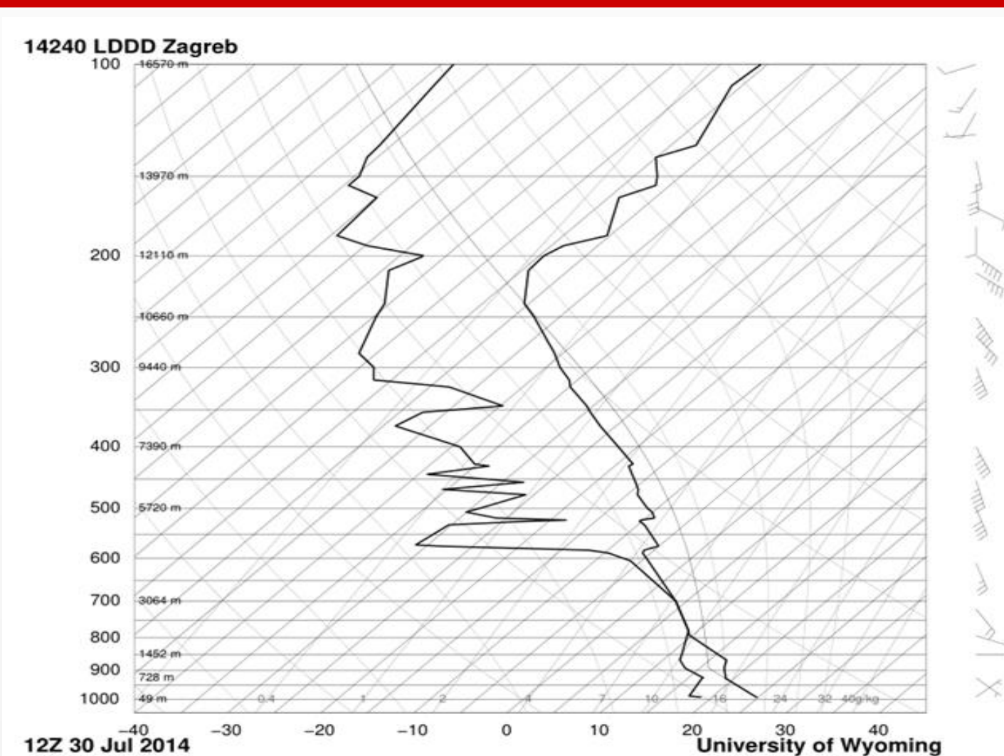
Figure 2: Sounding from Zagreb, Croatia (30.7.2014, 12 UTC) . CAPE = 857.7 J kg-1, LI = -2.65, K = 37,60 indicate a strong potential for convective activity. Freezing level is at 650 hPa and cloud base at 800 hPa. Strong dew point depression begins above 600 hPa.
